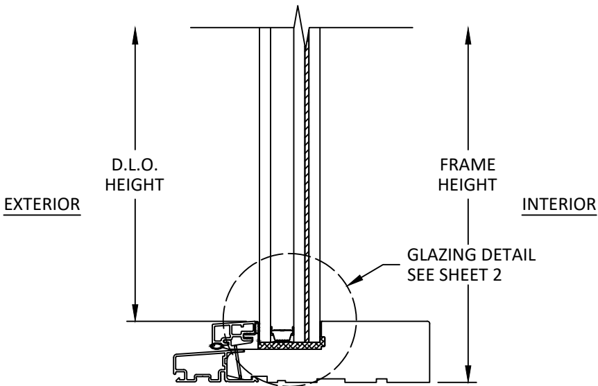
B 5 VERTICAL SECTION SILL INSULATED GLASS SHOWN
