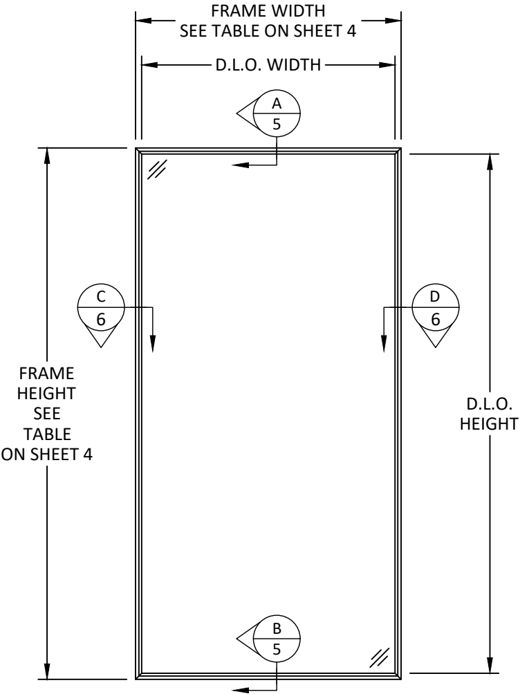
TYPICAL ELEVATION
