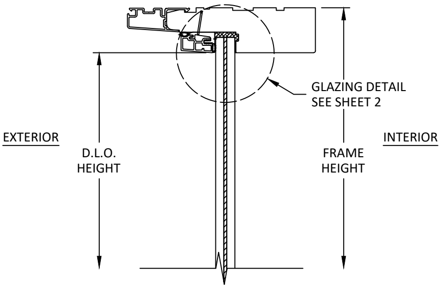
A 5 VERTICAL SECTION HEAD MONO. GLASS SHOWN
