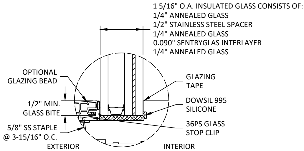
GLAZING DETAIL G3
