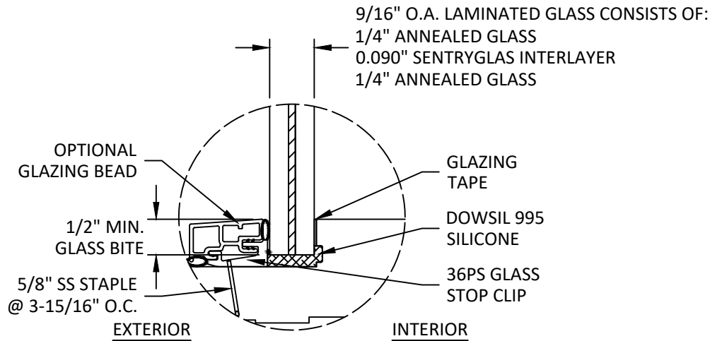
GLAZING DETAIL G1
