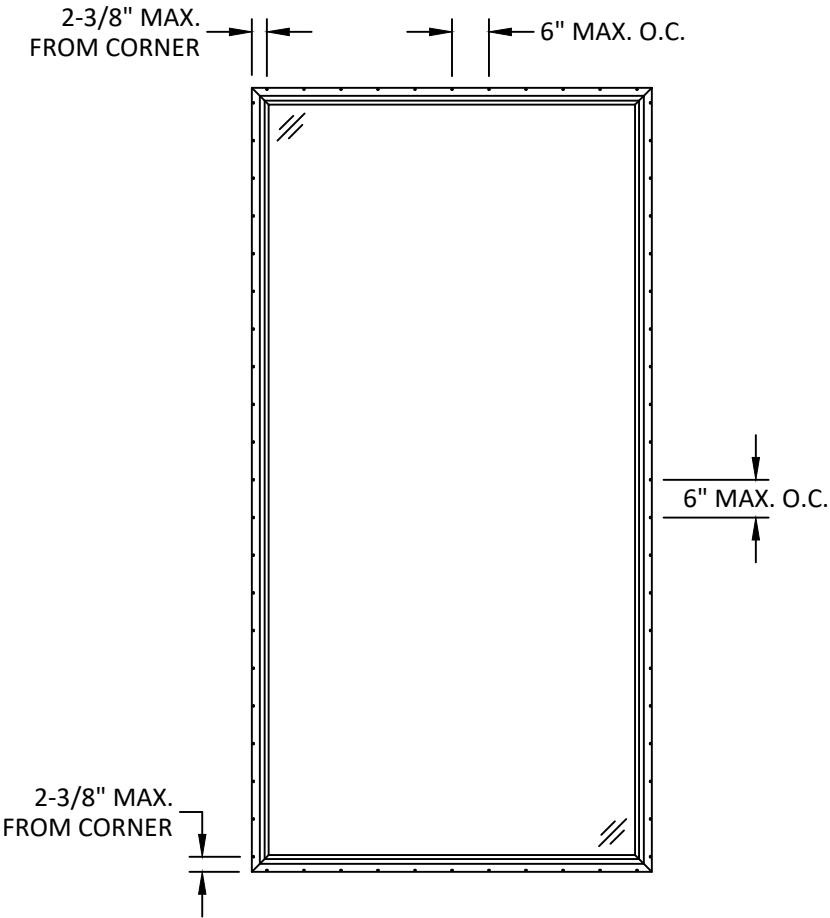
ANCHOR LAYOUT NAILING FLANGE
