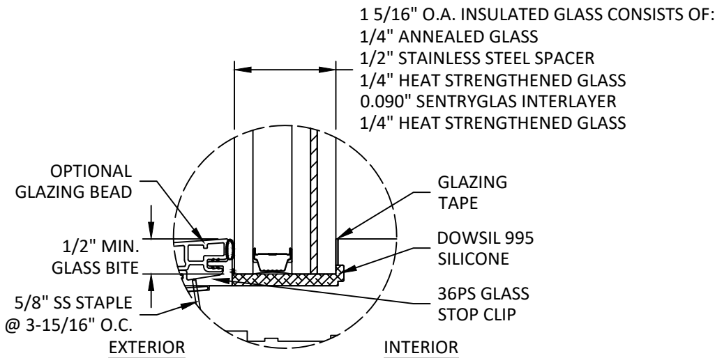
GLAZING DETAIL G4
